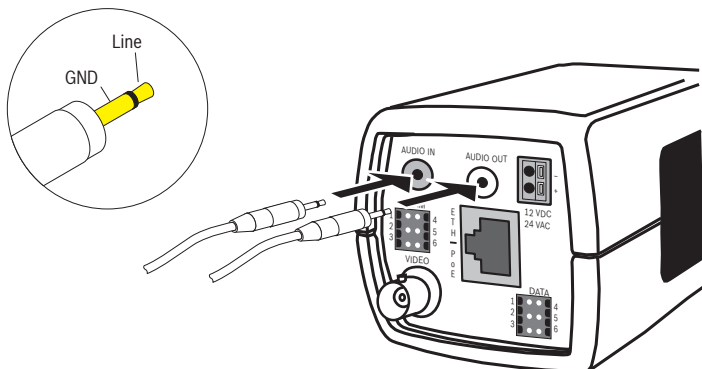
Figure 5.4 Audio connectors
